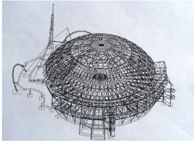
EXPO, HANNOVER 2000. 3D model of the structures
