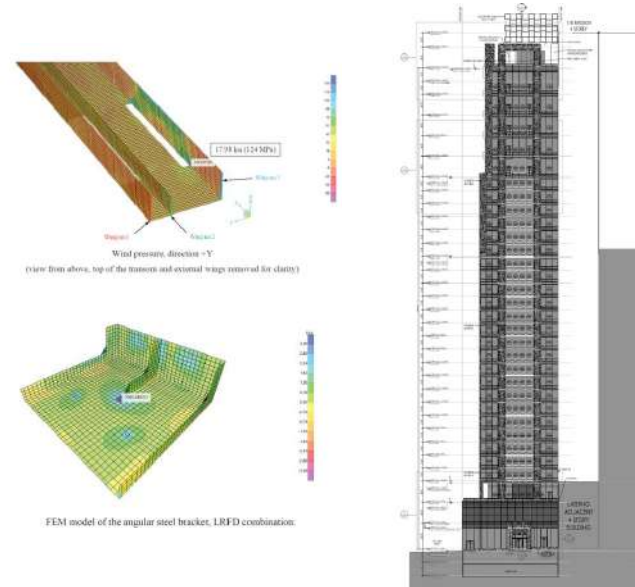
Structural design of curtain wall façade, floors 4-28 th . MADISON AVENUE RESIDENCES
