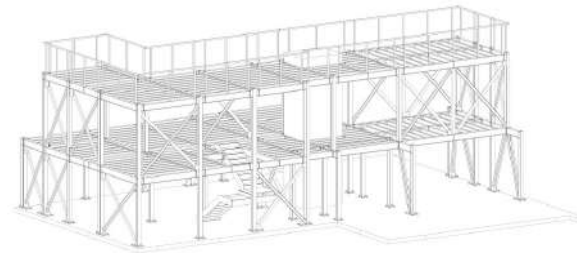
Upper storeys addition HOTEL MARCO POLO Jesolo - (Venezia) 3D Model
