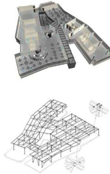
Upper storeys addition HOTEL RINAS ALBANIA 3D model
