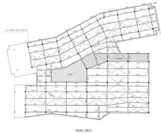
Upper storeys addition HOTEL RINAS ALBANIA Drawing
