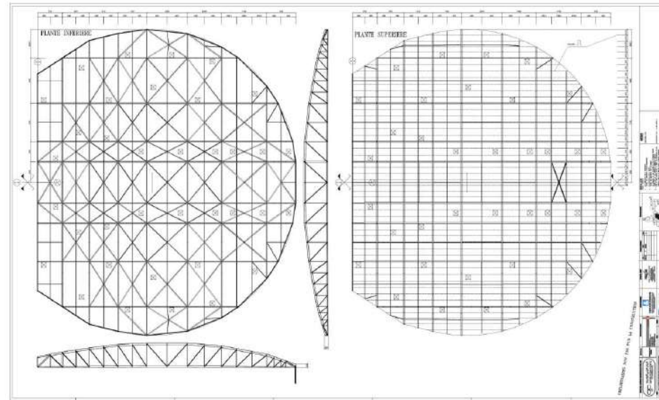
CENTRE INTERNATIONAL CONFERENCES CIC algér Block T4 - Drawing
