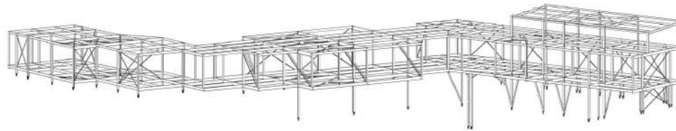
Upper storeys addition HOTEL ASTORIA Grado - (Gorizia). 3D Model
